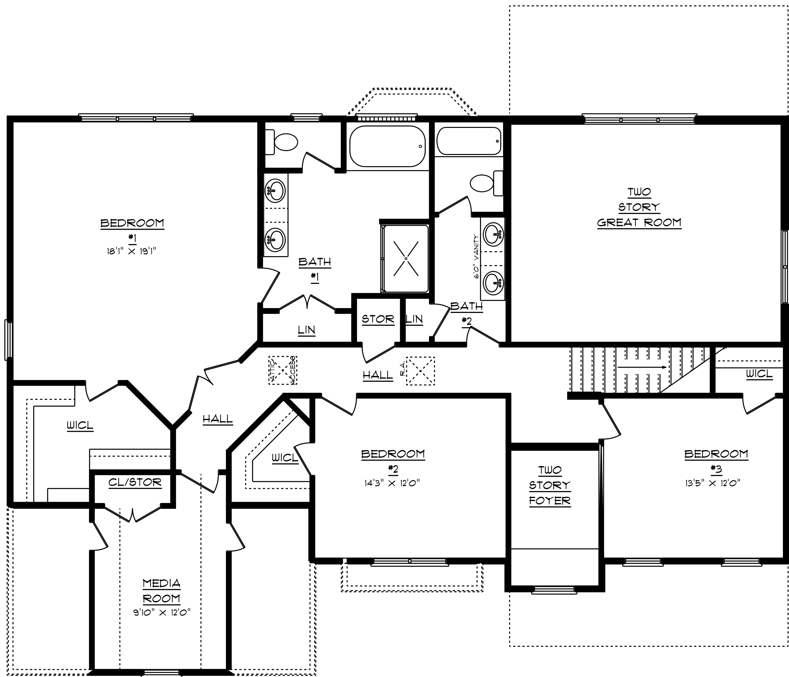
SECOND FLOOR
